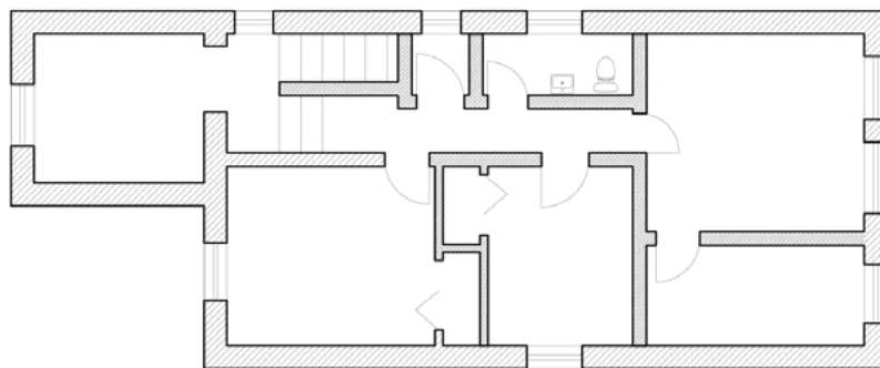
SECOND FLOOR APARTMENT PLAN AREA: 1,237 SQFT
